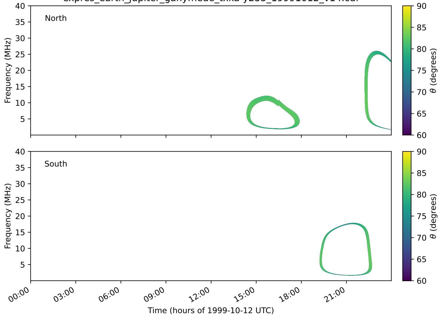
expres_earth_jupiter_ganymede_txka-y235_19991012_v14.cdf
