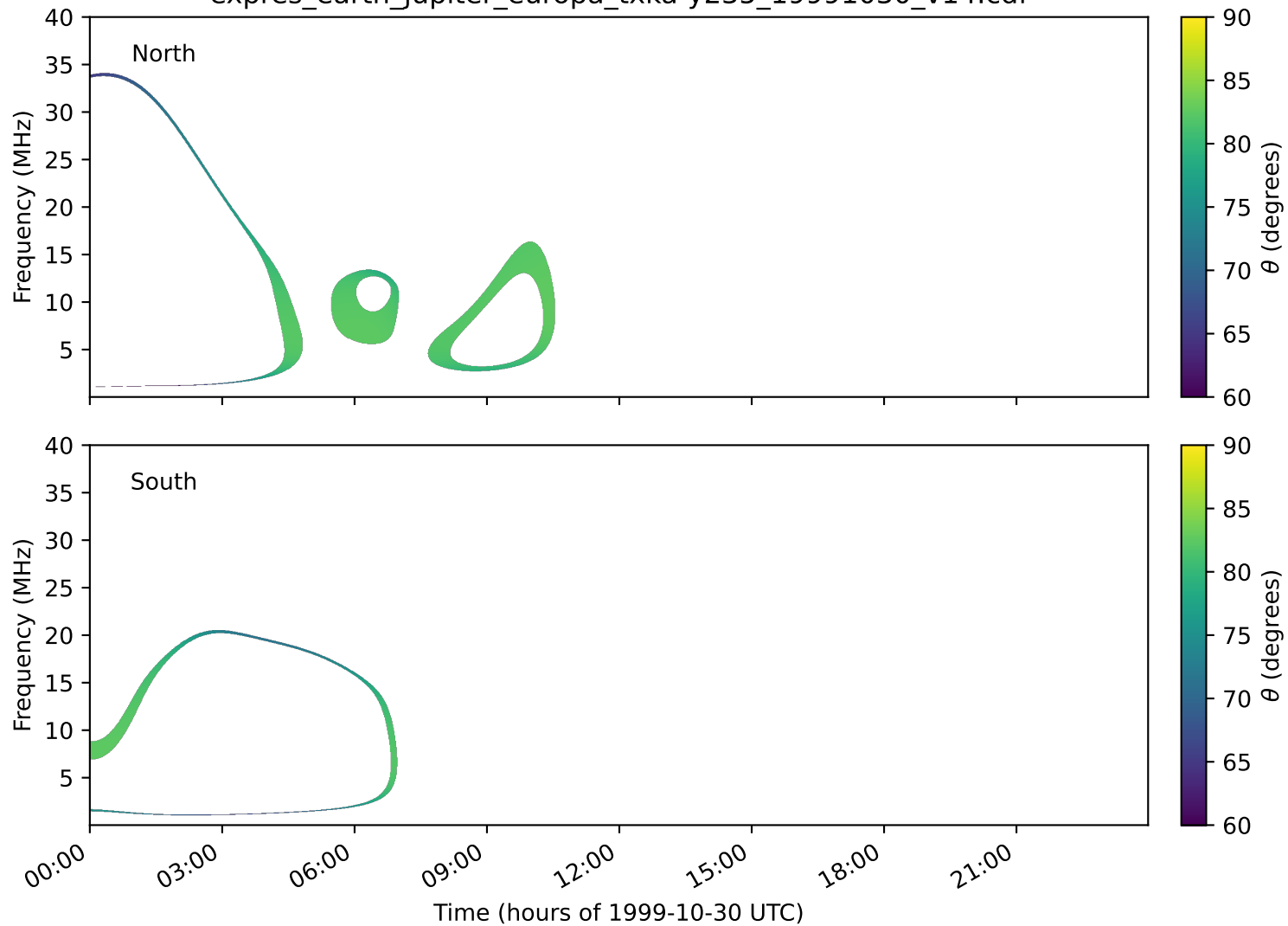
expres_earth_jupiter_europa_txka-y235_19991030_v14.cdf
