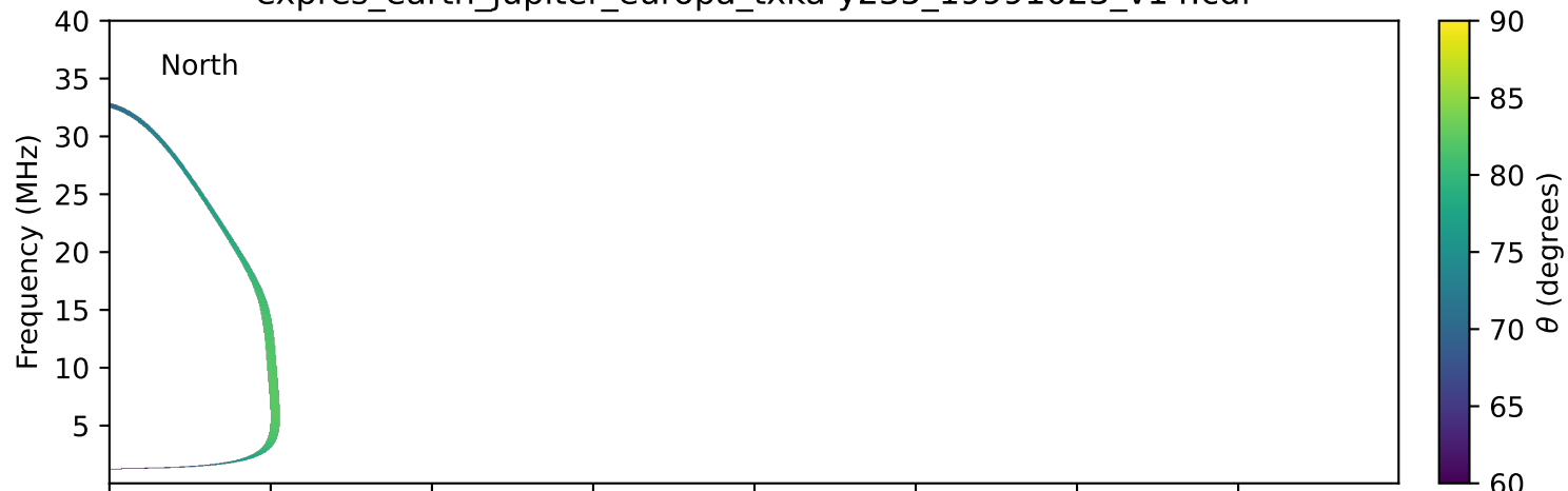
expres_earth_jupiter_europa_txka-y235_19991023_v14.cdf
