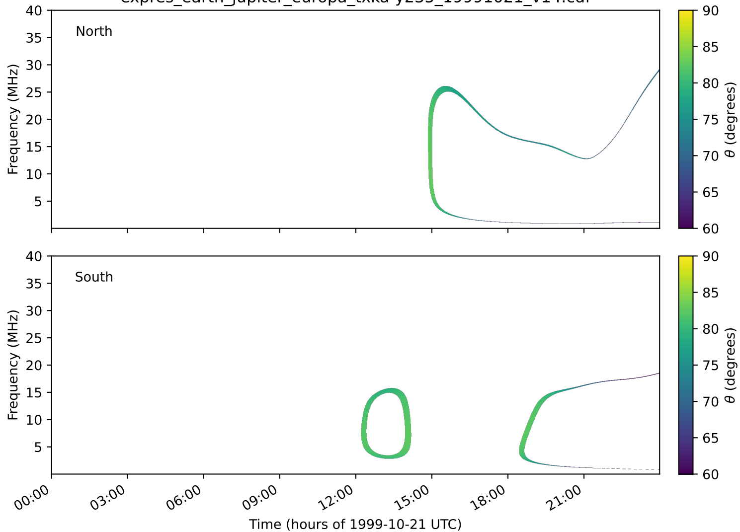
expres_earth_jupiter_europa_txka-y235_19991021_v14.cdf
