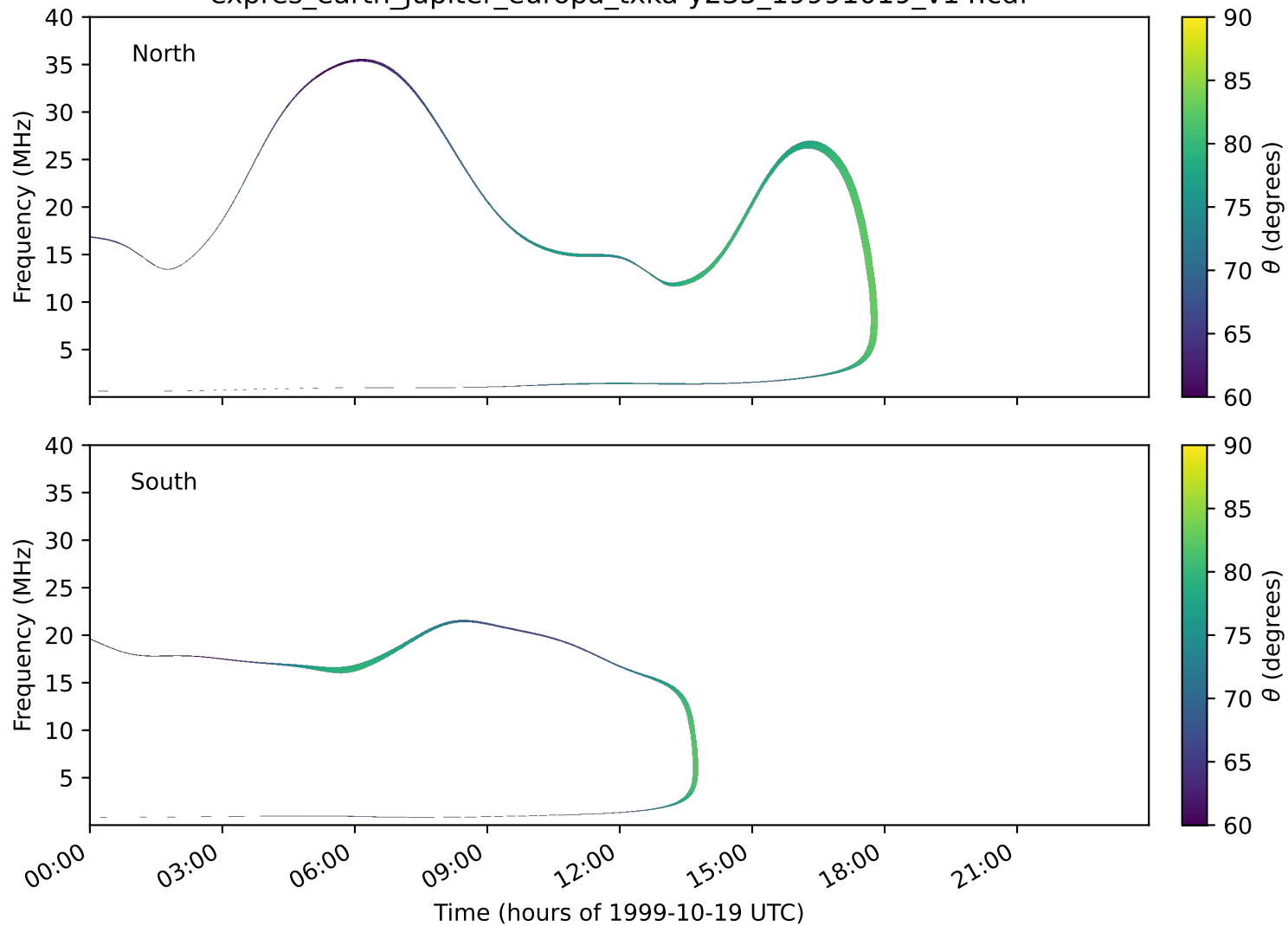
expres_earth_jupiter_europa_txka-y235_19991019_v14.cdf
