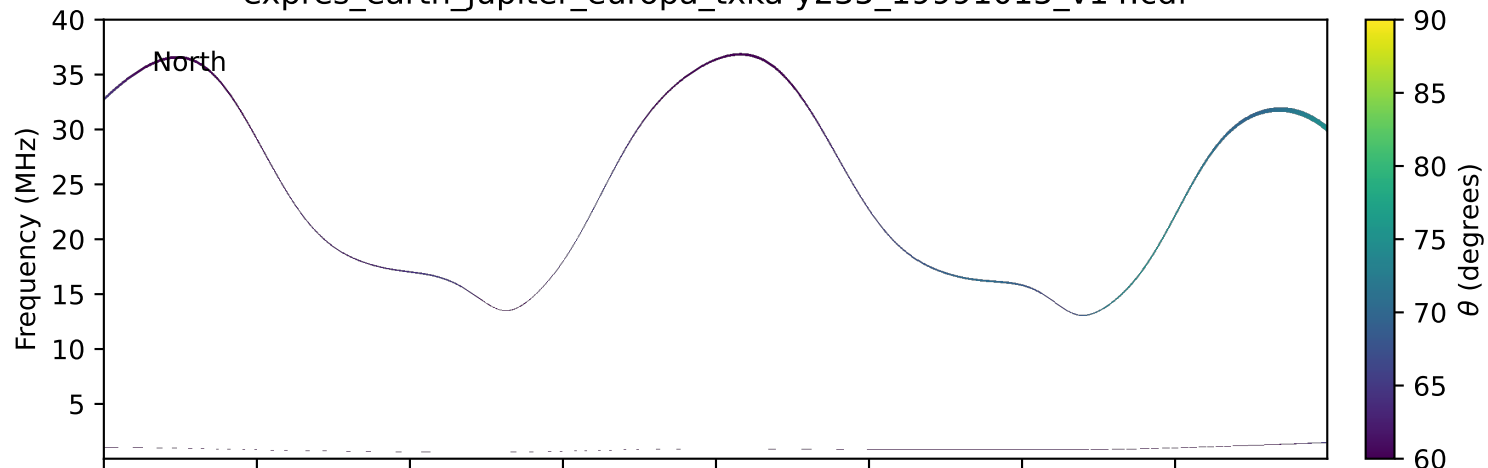
expres_earth_jupiter_europa_txka-y235_19991015_v14.cdf
