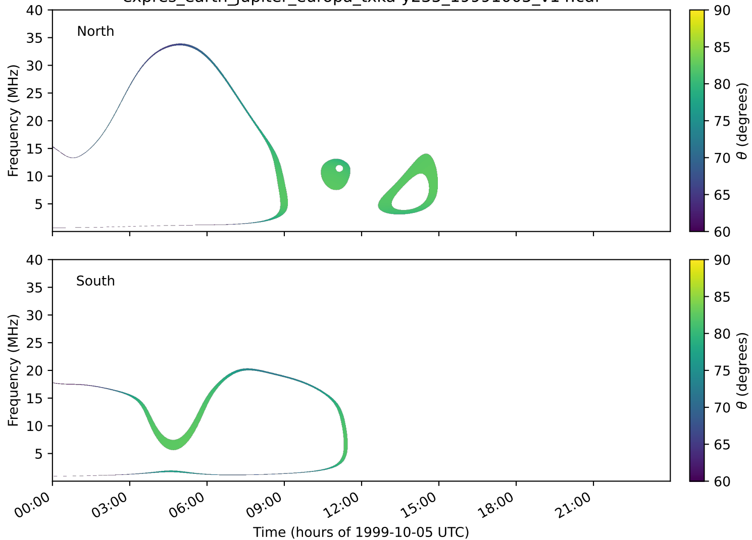
expres_earth_jupiter_europa_txka-y235_19991005_v14.cdf
