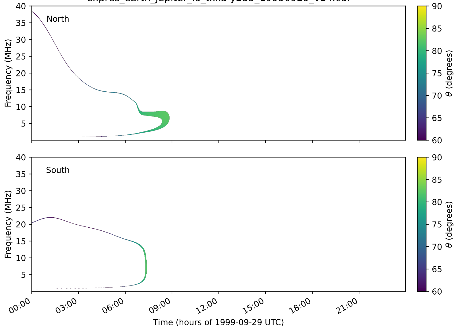
expres_earth_jupiter_io_txka-y235_19990929_v14.cdf
