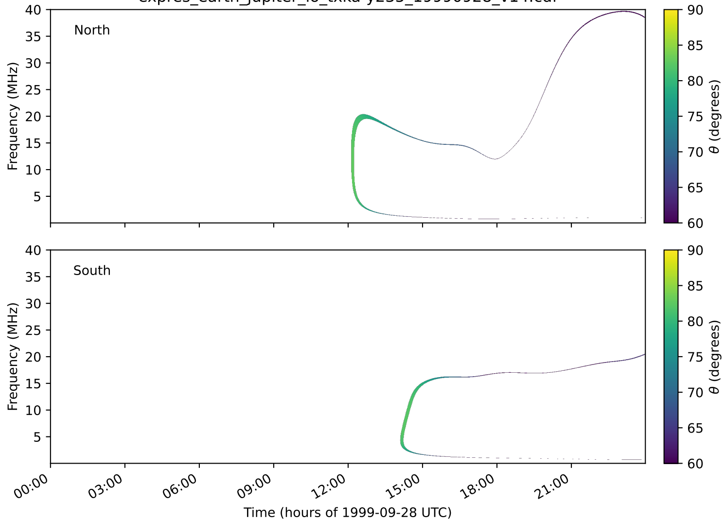
expres_earth_jupiter_io_txka-y235_19990928_v14.cdf
