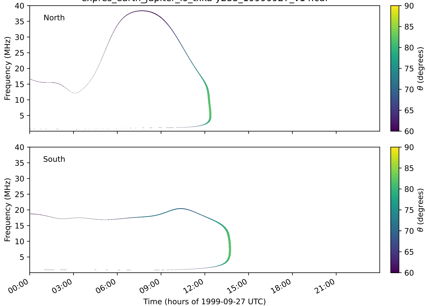
expres_earth_jupiter_io_txka-y235_19990927_v14.cdf
