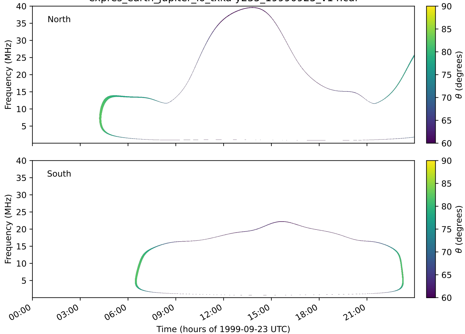
expres_earth_jupiter_io_txka-y235_19990923_v14.cdf
