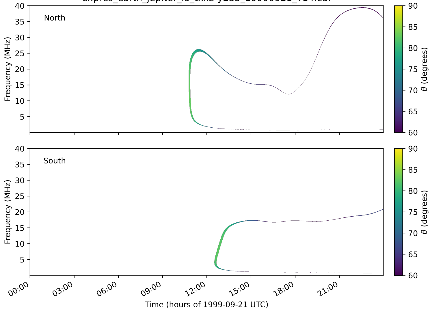
expres_earth_jupiter_io_txka-y235_19990921_v14.cdf
