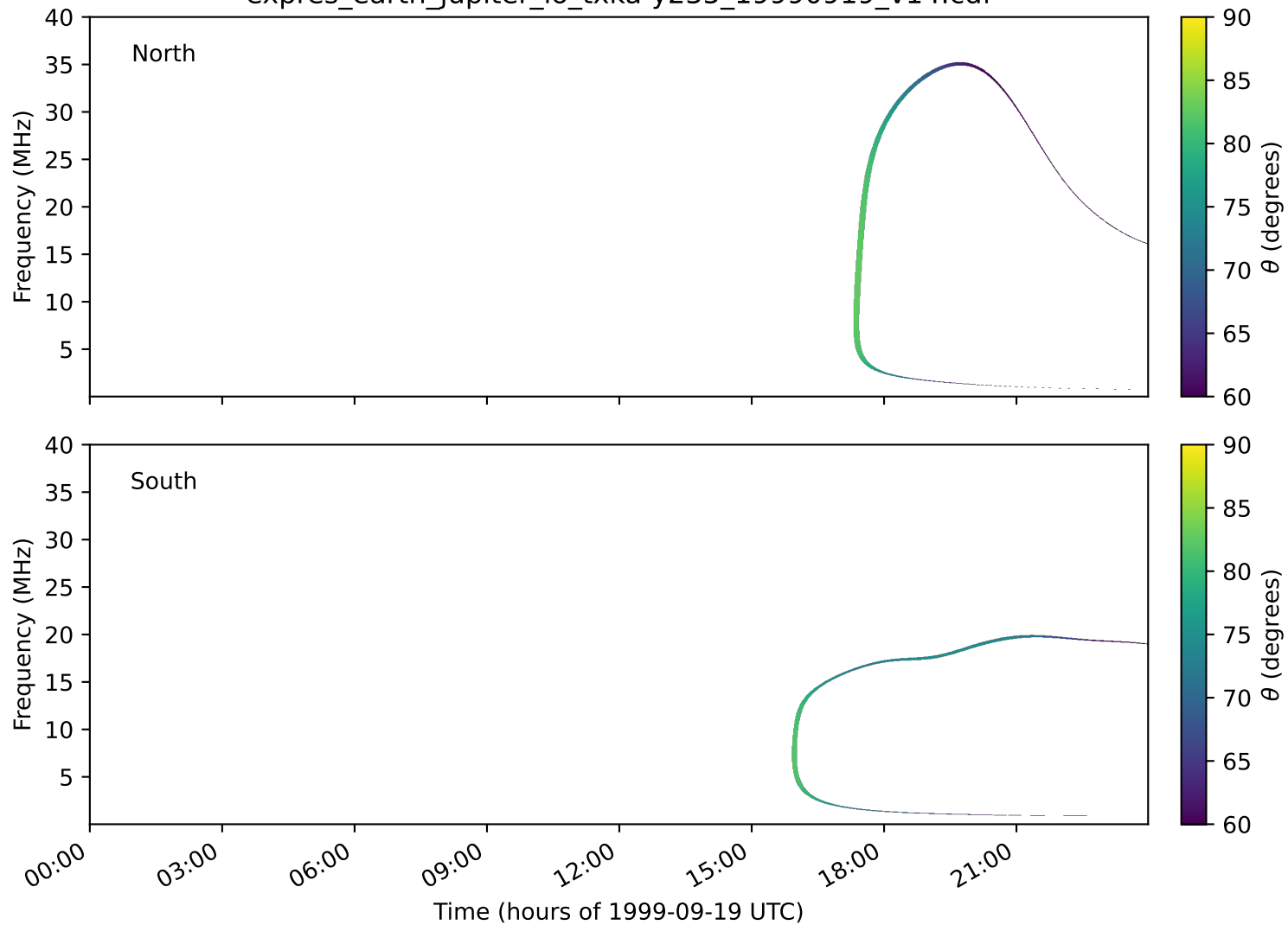
expres_earth_jupiter_io_txka-y235_19990919_v14.cdf
