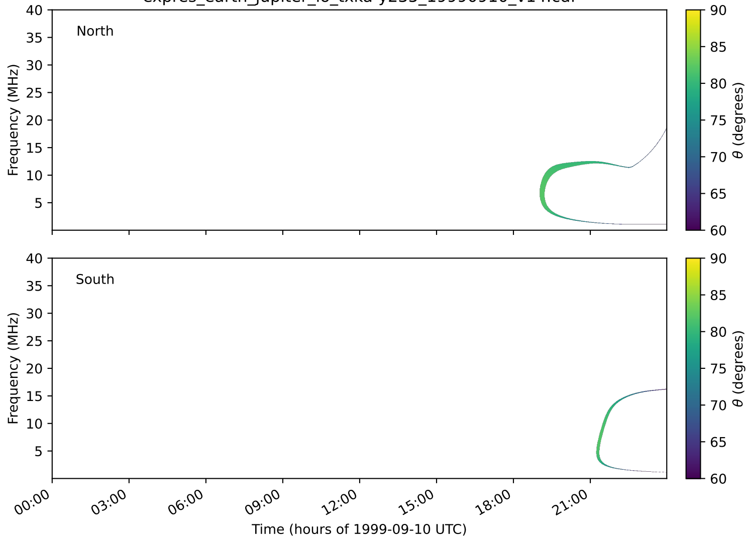
expres_earth_jupiter_io_txka-y235_19990910_v14.cdf
