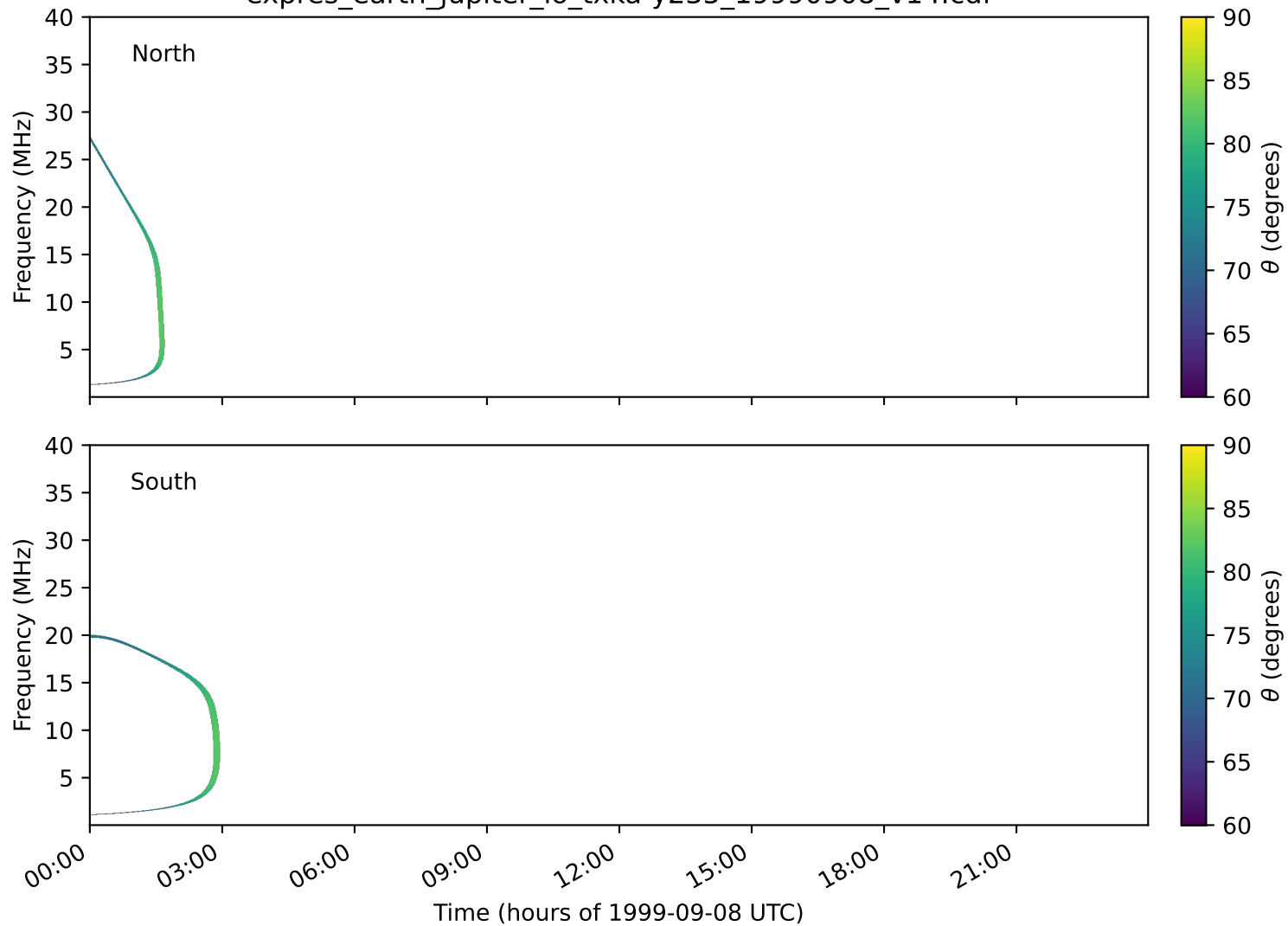
expres_earth_jupiter_io_txka-y235_19990908_v14.cdf
