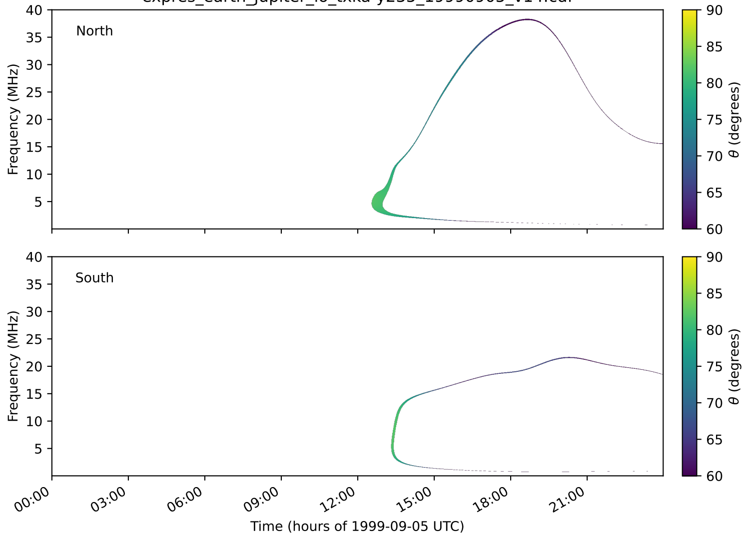
expres_earth_jupiter_io_txka-y235_19990905_v14.cdf
