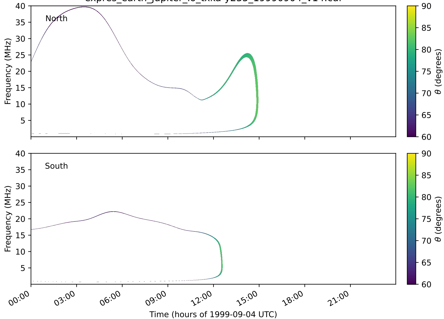
expres_earth_jupiter_io_txka-y235_19990904_v14.cdf
