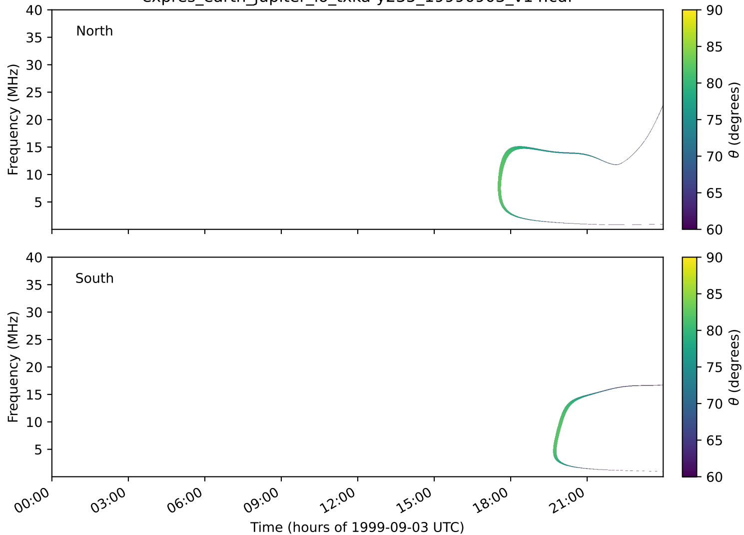
expres_earth_jupiter_io_txka-y235_19990903_v14.cdf
