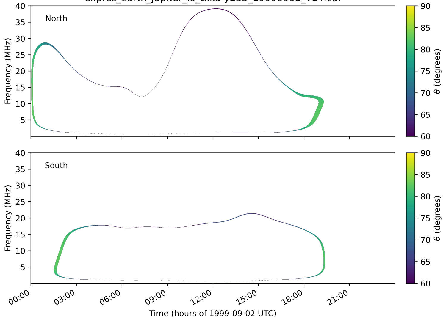
expres_earth_jupiter_io_txka-y235_19990902_v14.cdf
