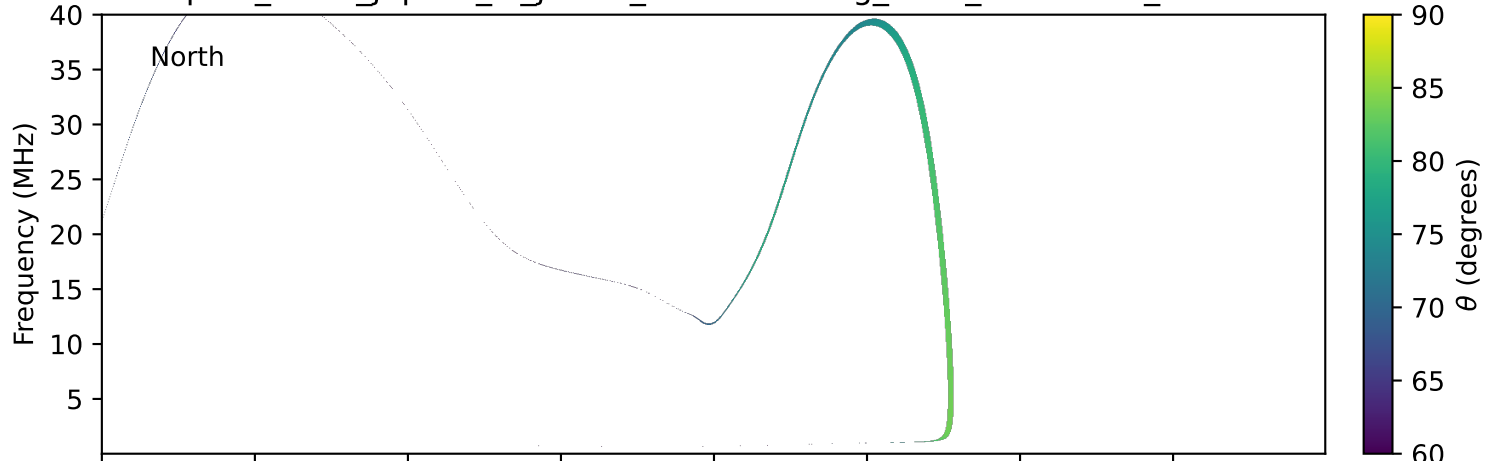
expres_earth_jupiter_io_jrm09_lossc-wid1deg_3kev_19990911_v11.cdf
