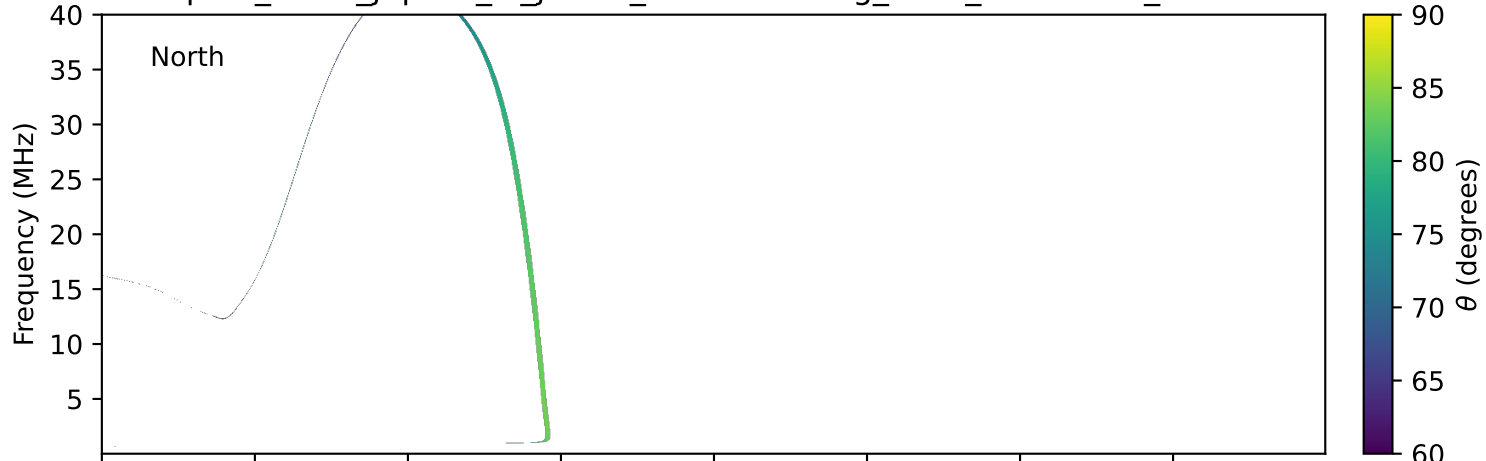
expres_earth_jupiter_io_jrm09_lossc-wid1deg_3kev_19990906_v11.cdf
