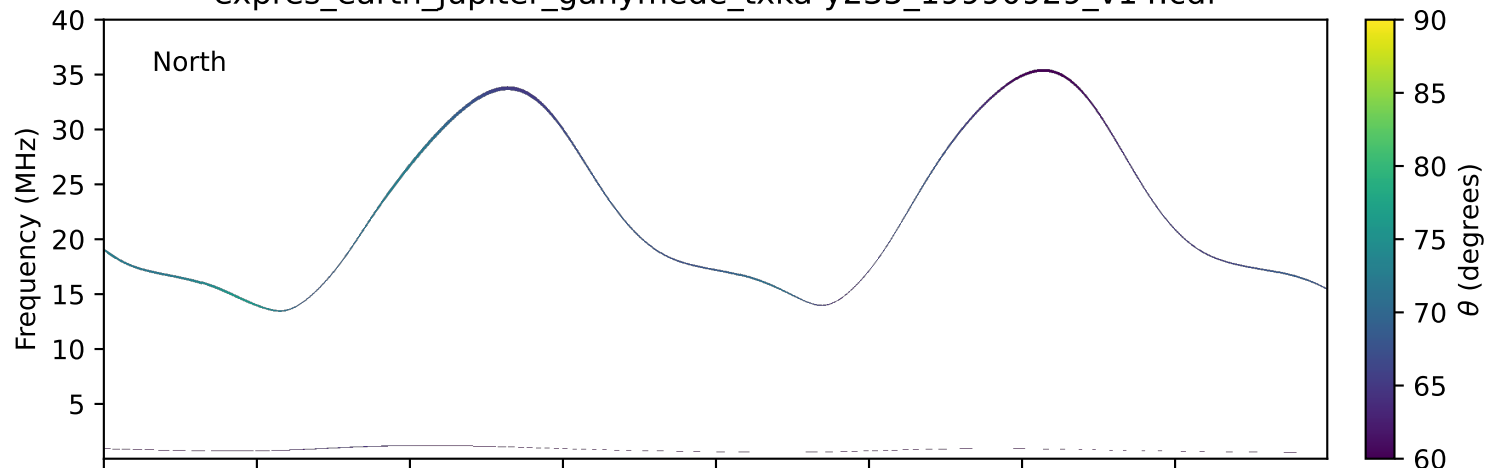
expres_earth_jupiter_ganymede_txka-y235_19990929_v14.cdf
