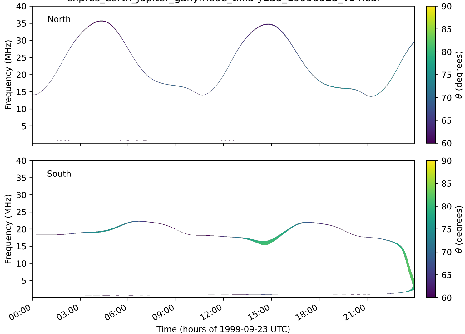
expres_earth_jupiter_ganymede_txka-y235_19990923_v14.cdf
