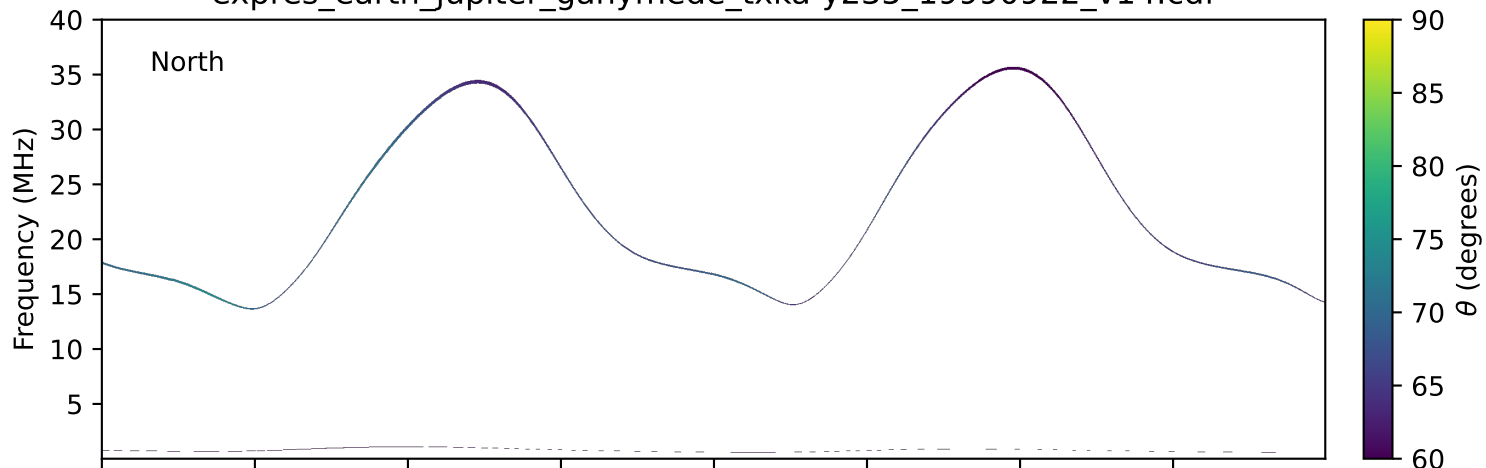
expres_earth_jupiter_ganymede_txka-y235_19990922_v14.cdf
