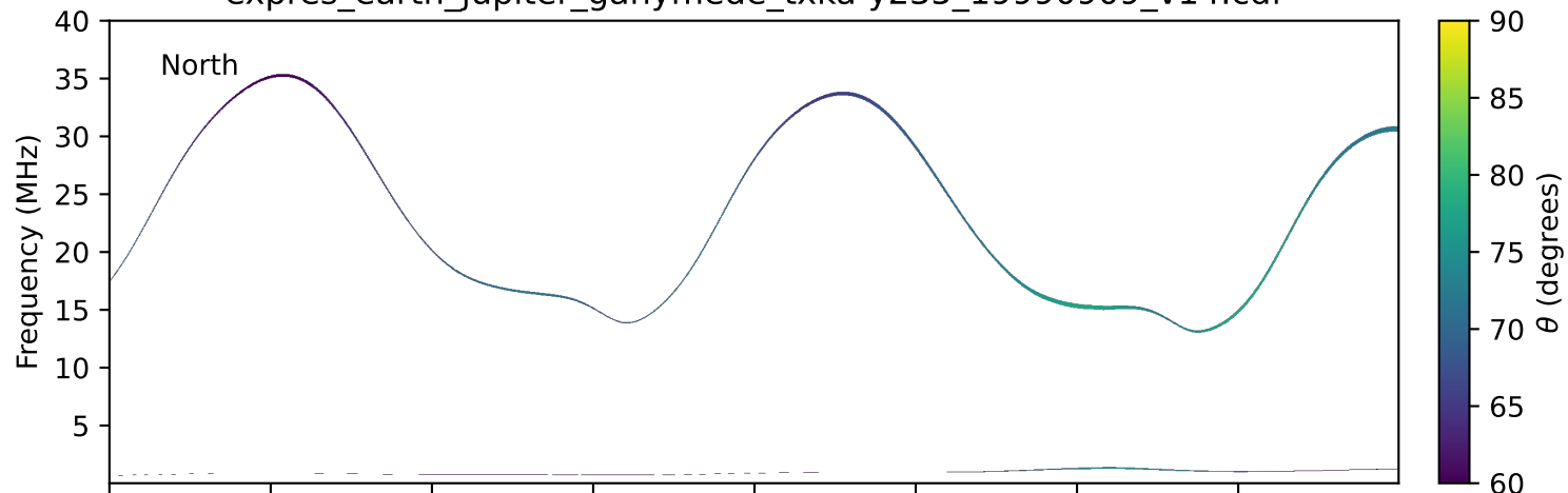
expres_earth_jupiter_ganymede_txka-y235_19990909_v14.cdf
