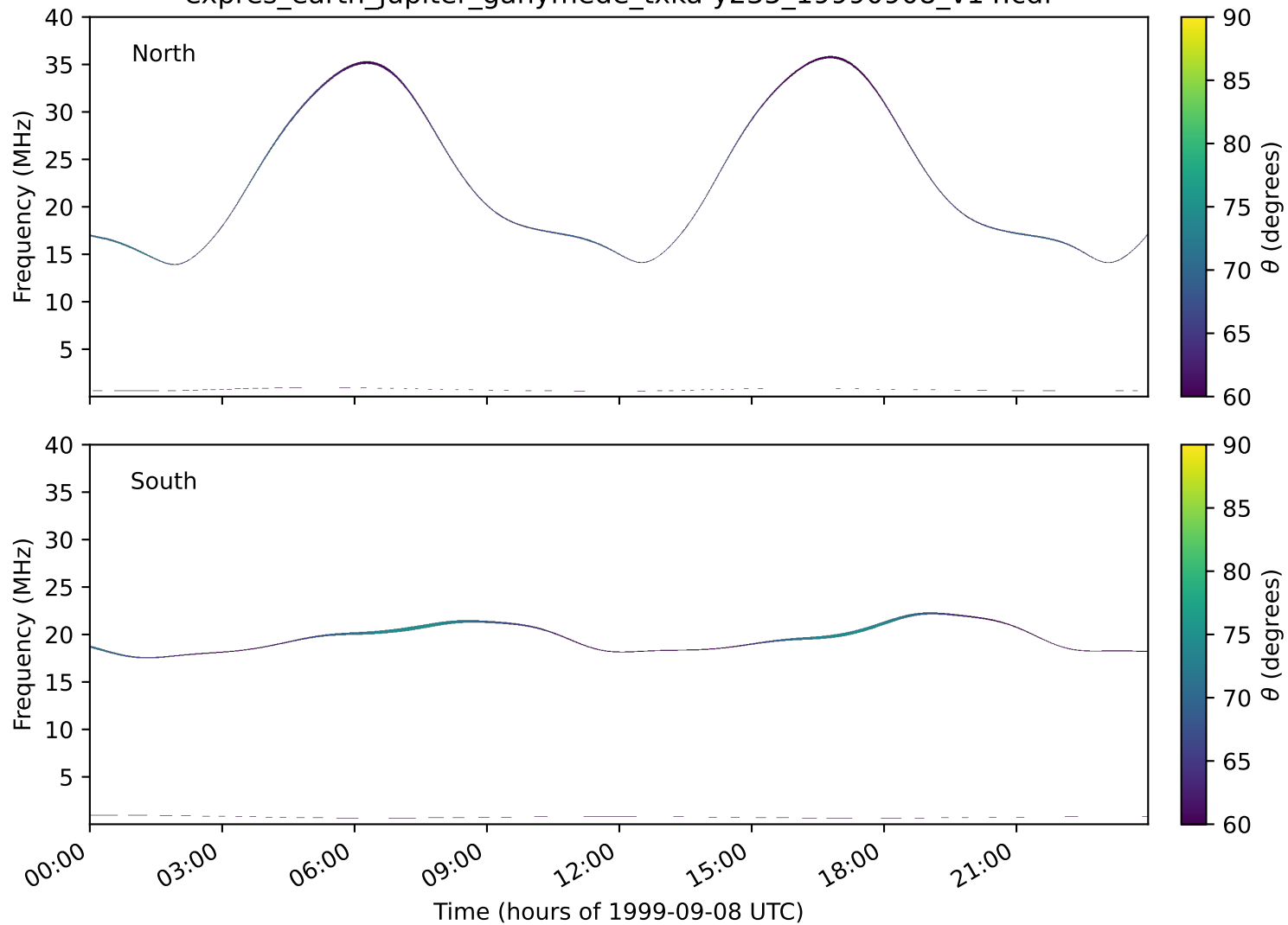
expres_earth_jupiter_ganymede_txka-y235_19990908_v14.cdf
