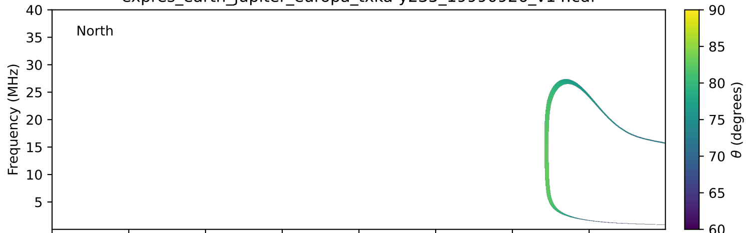
expres_earth_jupiter_europa_txka-y235_19990926_v14.cdf
