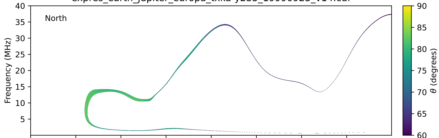
expres_earth_jupiter_europa_txka-y235_19990923_v14.cdf
