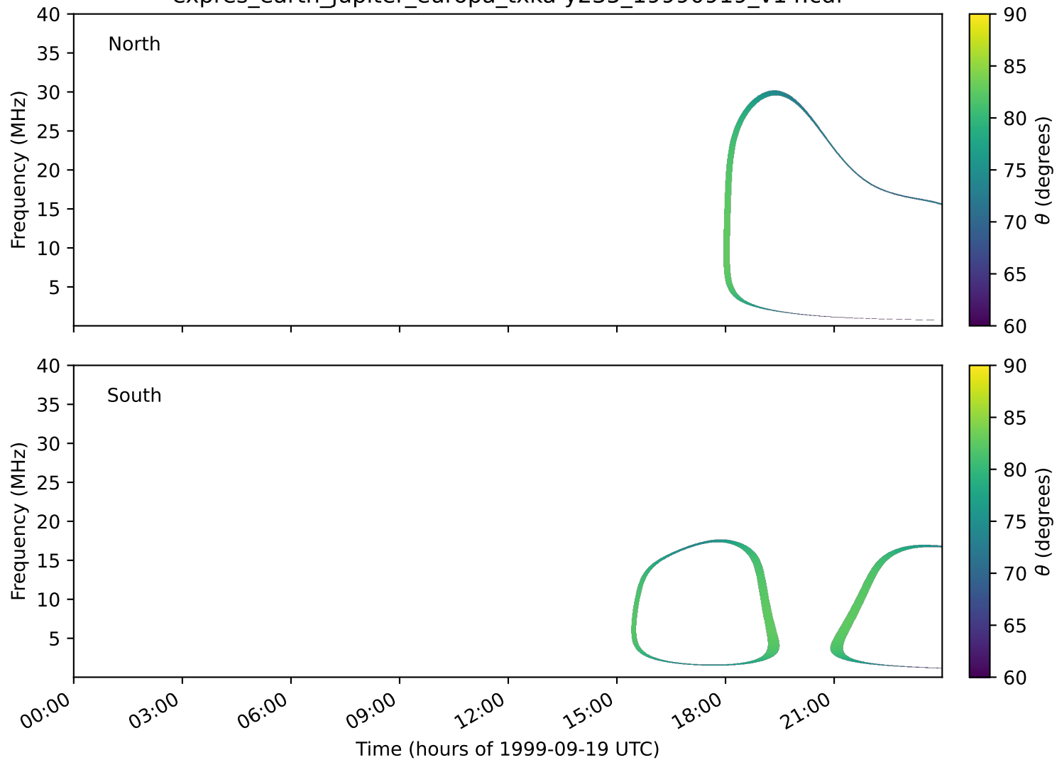
expres_earth_jupiter_europa_txka-y235_19990919_v14.cdf
