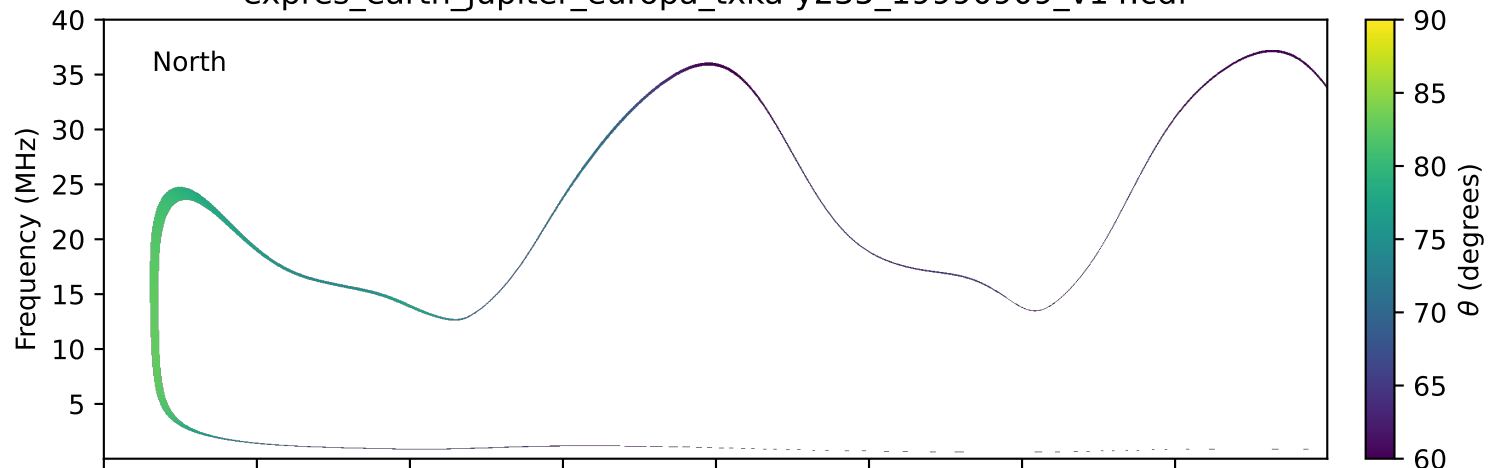
expres_earth_jupiter_europa_txka-y235_19990909_v14.cdf
