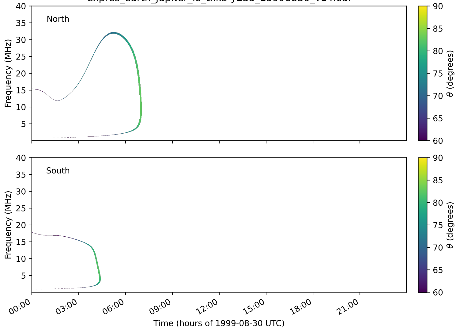
expres_earth_jupiter_io_txka-y235_19990830_v14.cdf
