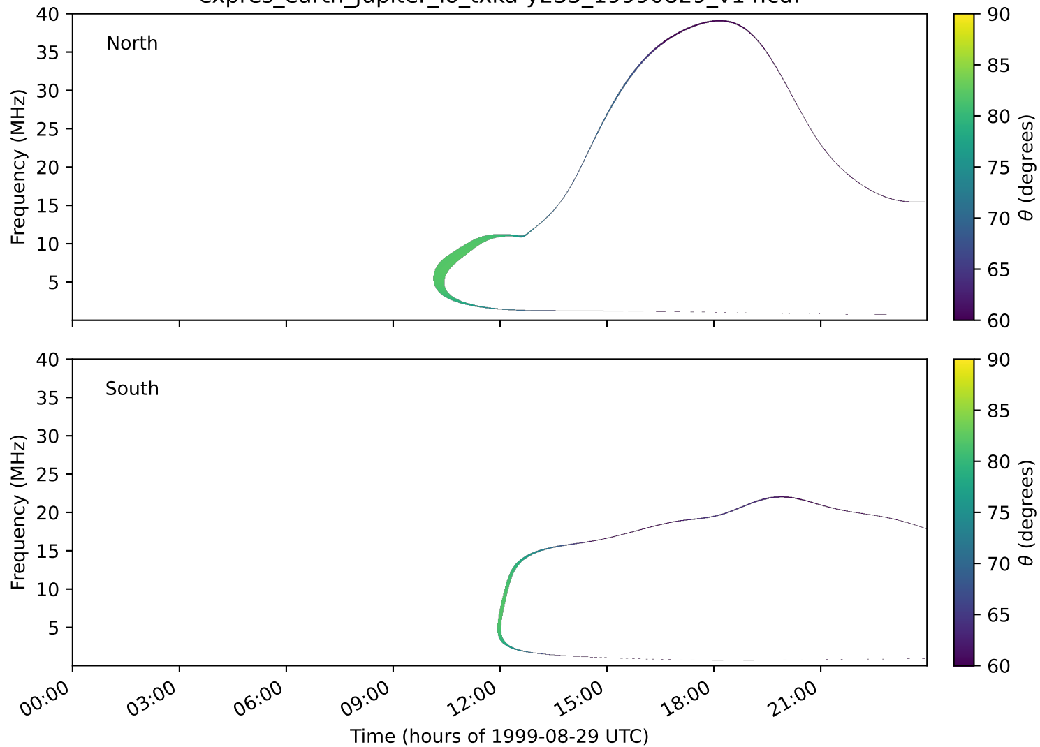
expres_earth_jupiter_io_txka-y235_19990829_v14.cdf
