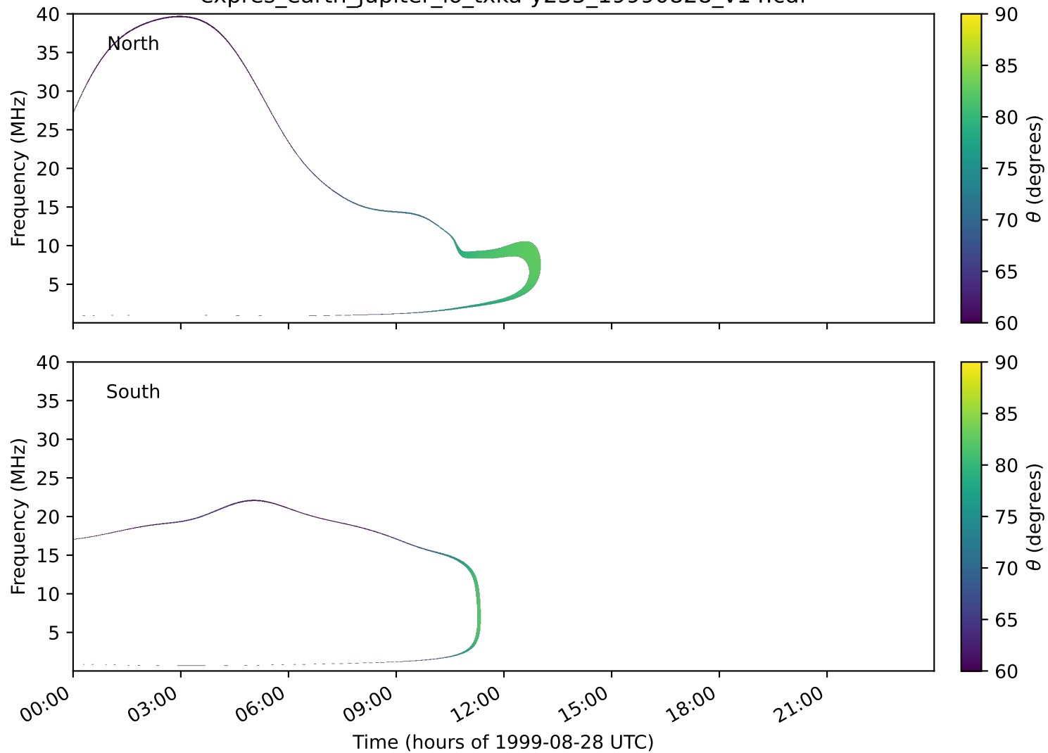
expres_earth_jupiter_io_txka-y235_19990828_v14.cdf
