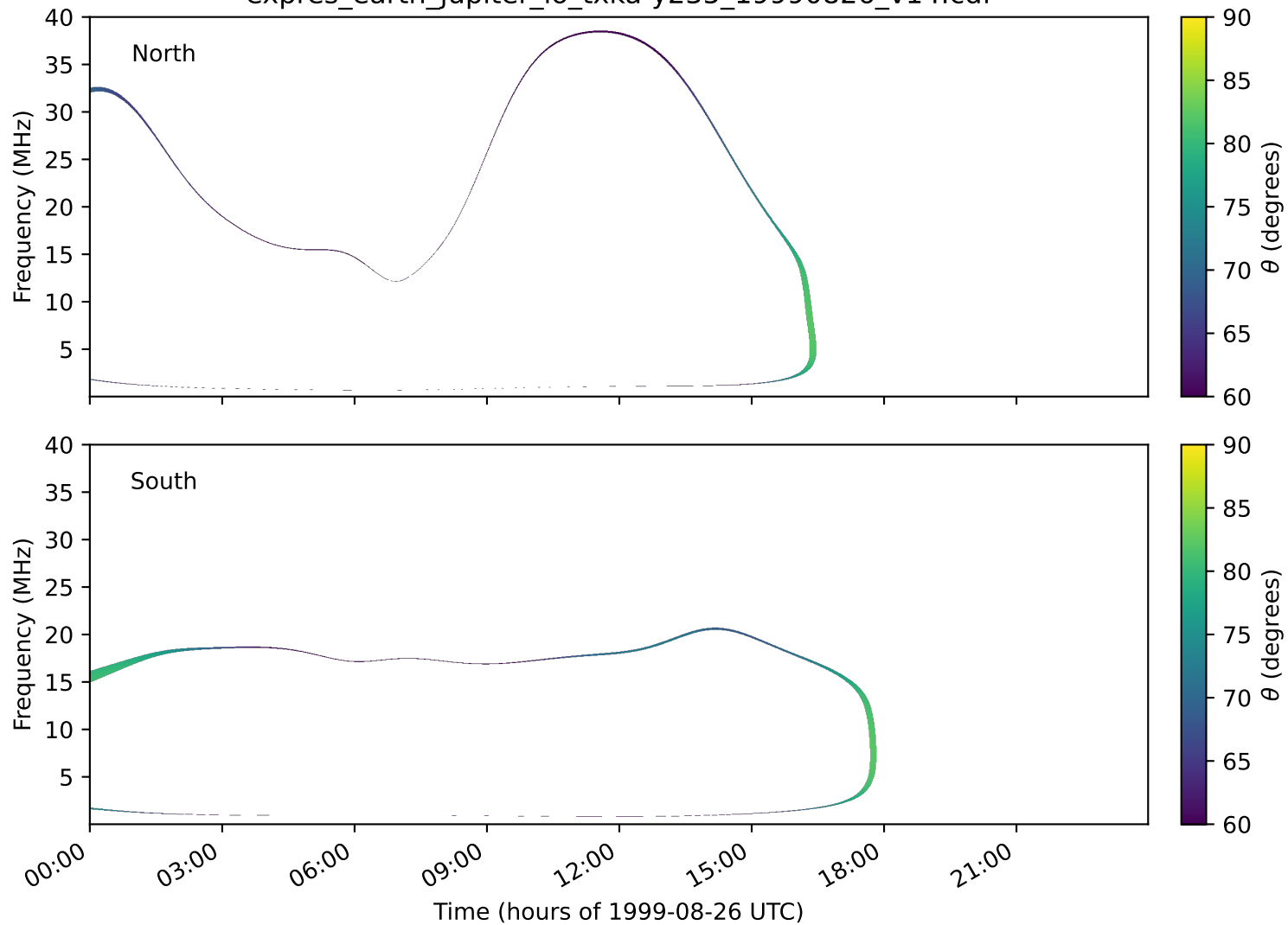
expres_earth_jupiter_io_txka-y235_19990826_v14.cdf
