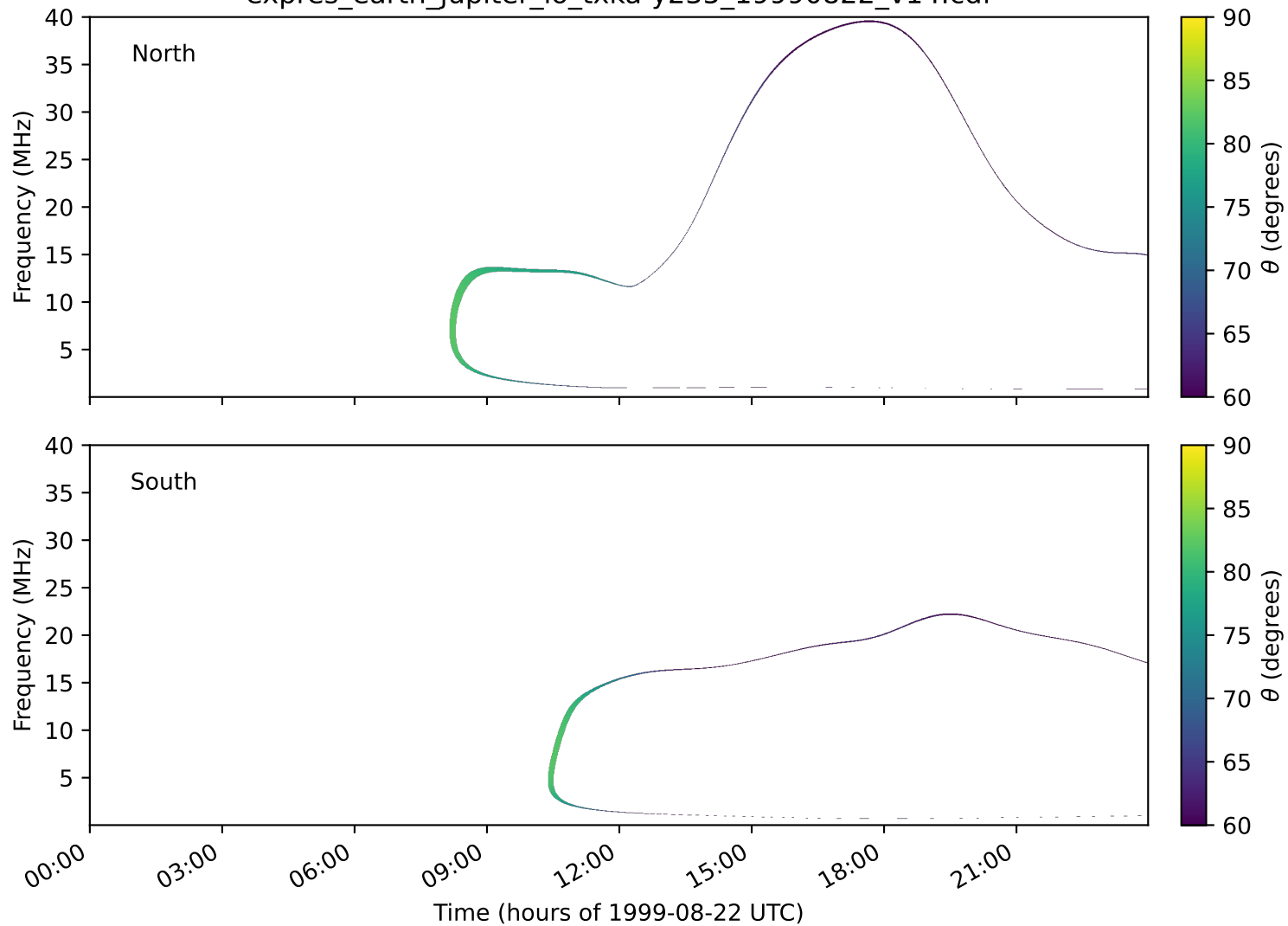
expres_earth_jupiter_io_txka-y235_19990822_v14.cdf
