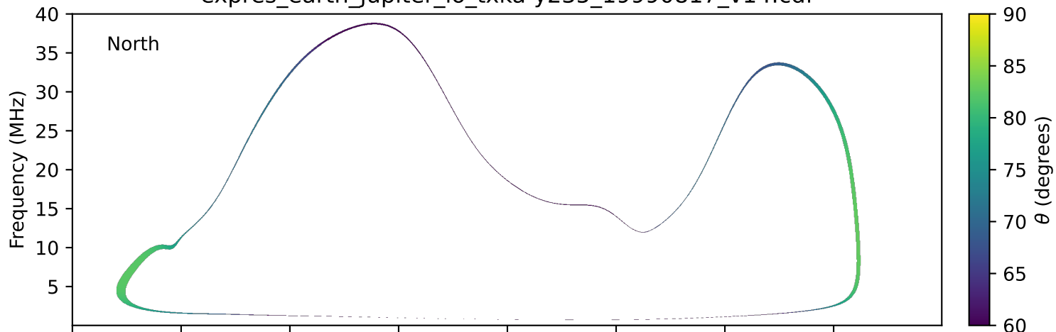
expres_earth_jupiter_io_txka-y235_19990817_v14.cdf
