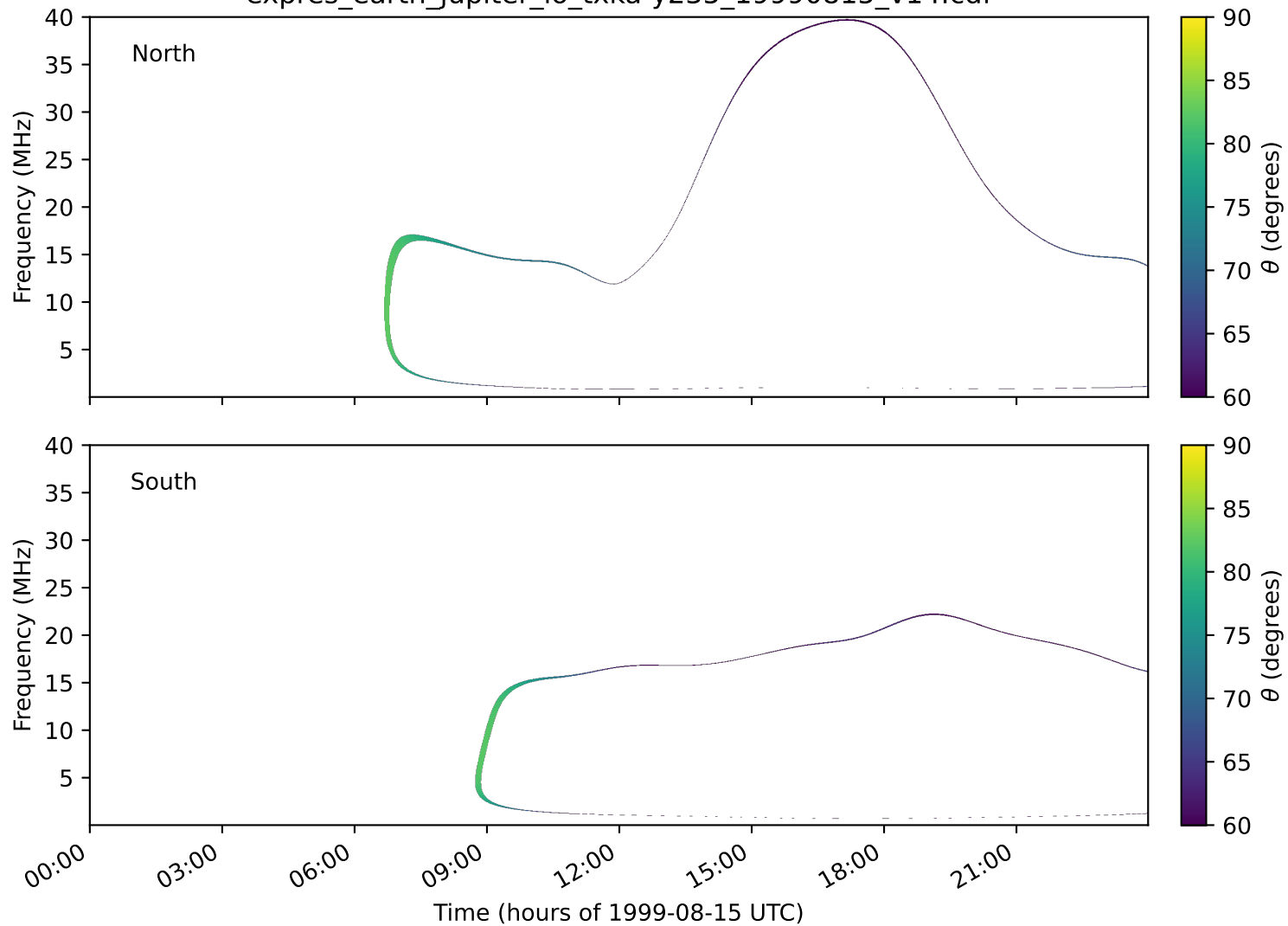
expres_earth_jupiter_io_txka-y235_19990815_v14.cdf
