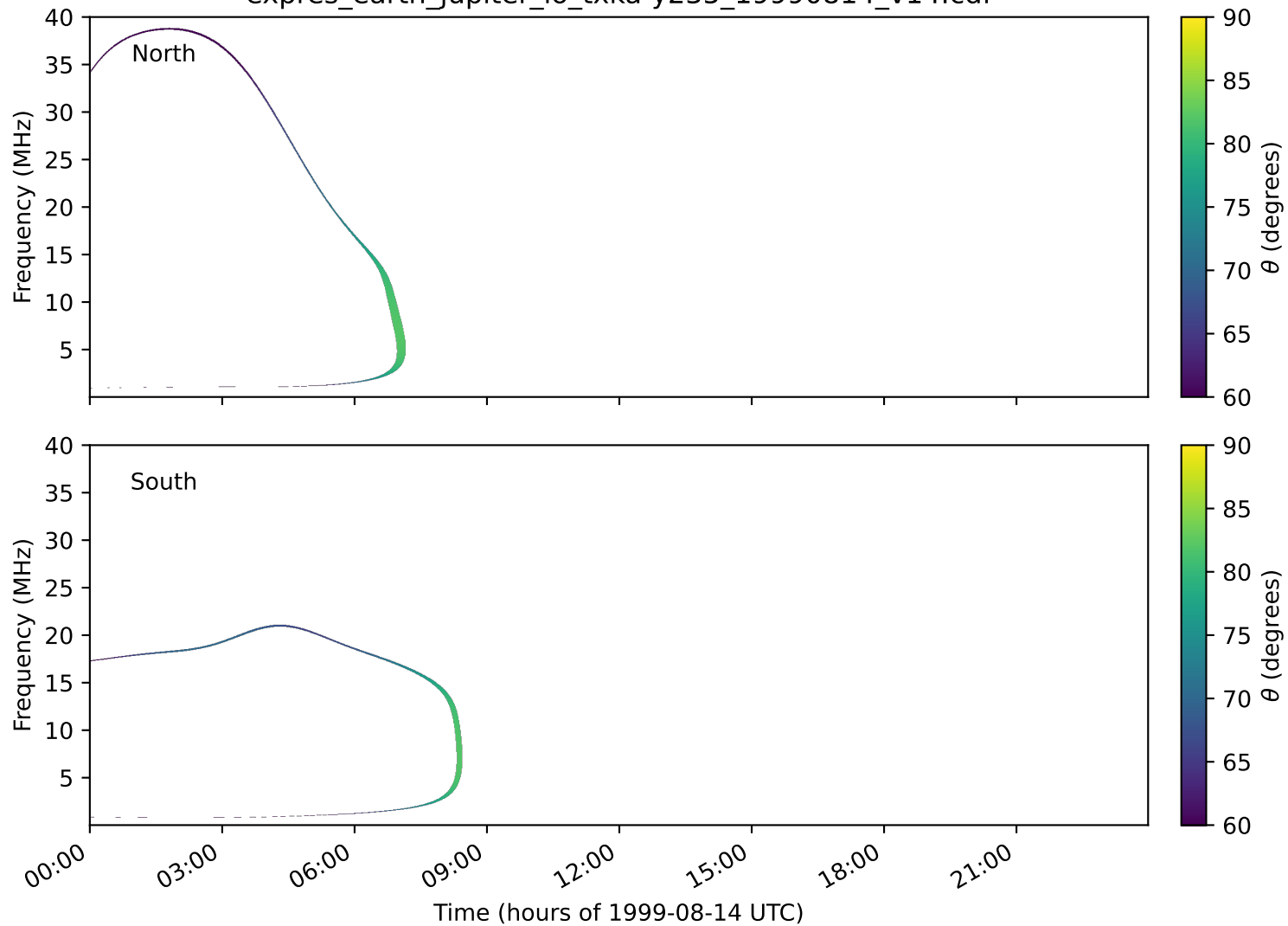
expres_earth_jupiter_io_txka-y235_19990814_v14.cdf
