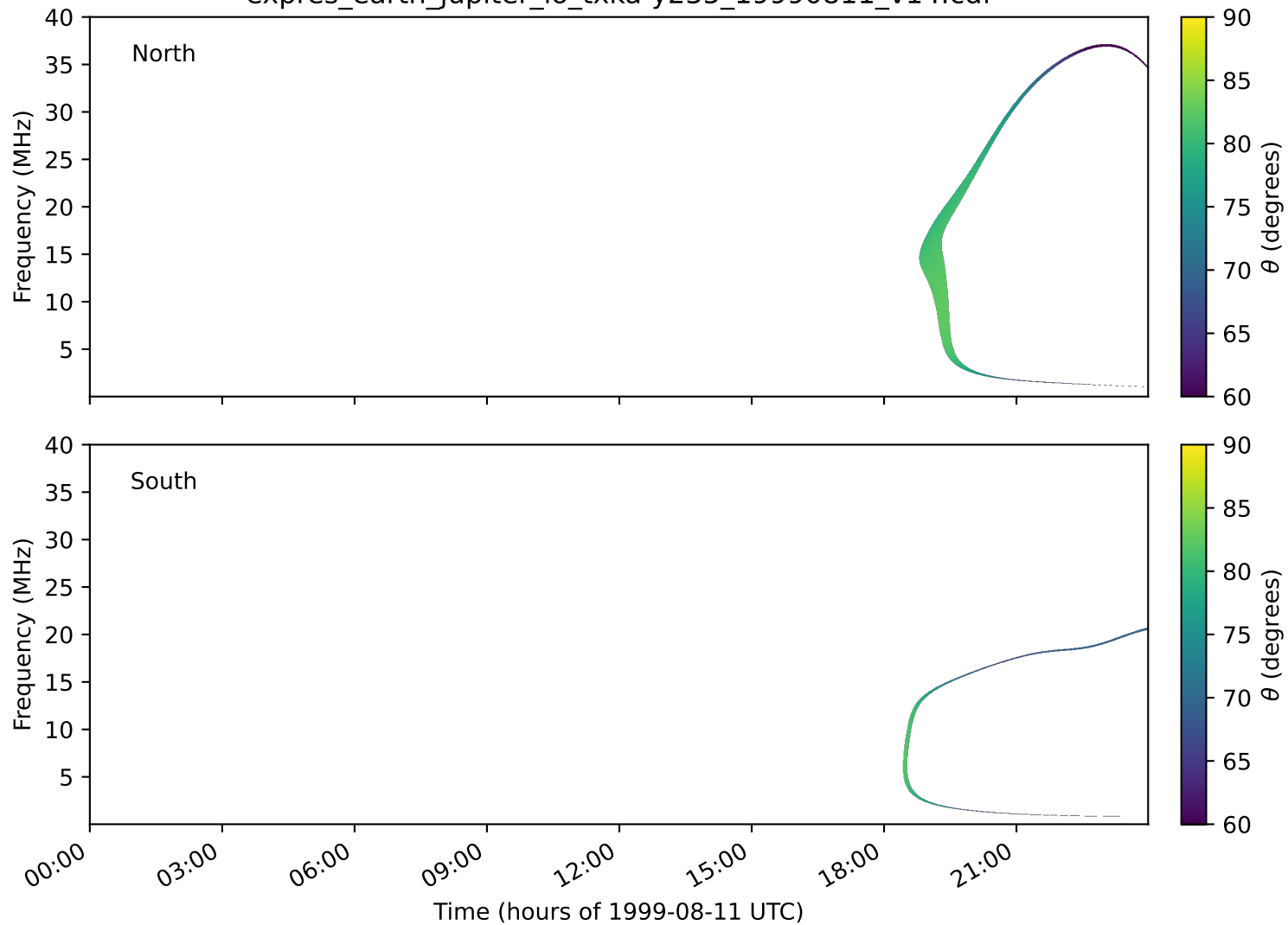
expres_earth_jupiter_io_txka-y235_19990811_v14.cdf
