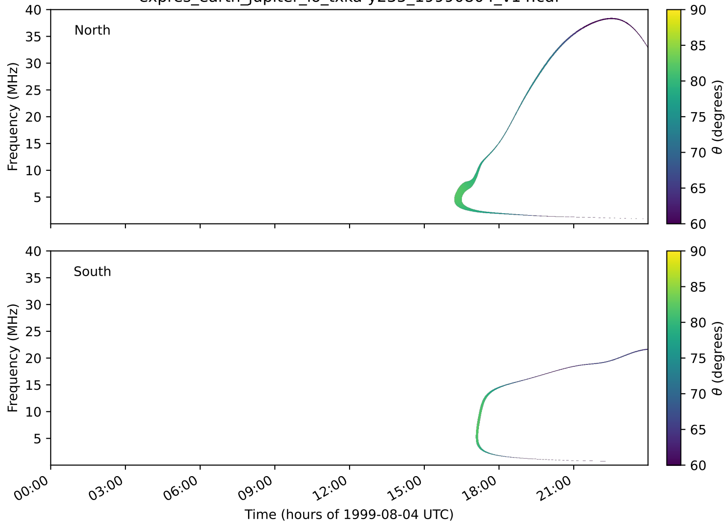
expres_earth_jupiter_io_txka-y235_19990804_v14.cdf
