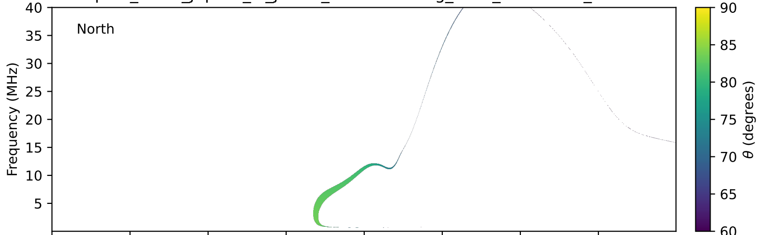
expres_earth_jupiter_io_jrm09_lossc-wid1deg_3kev_19990829_v11.cdf
