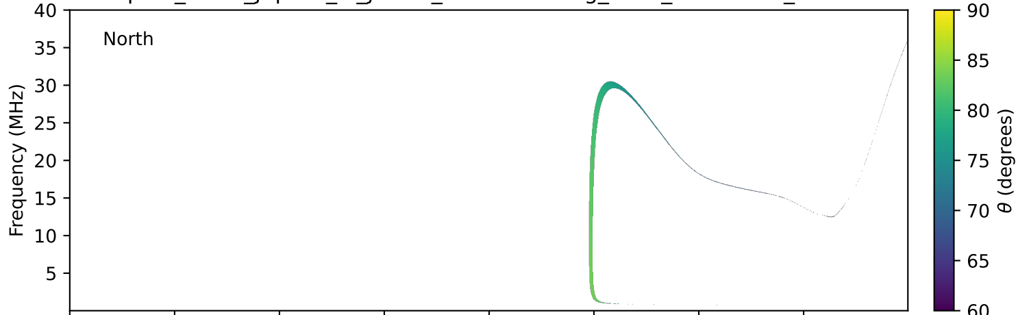
expres_earth_jupiter_io_jrm09_lossc-wid1deg_3kev_19990820_v11.cdf
