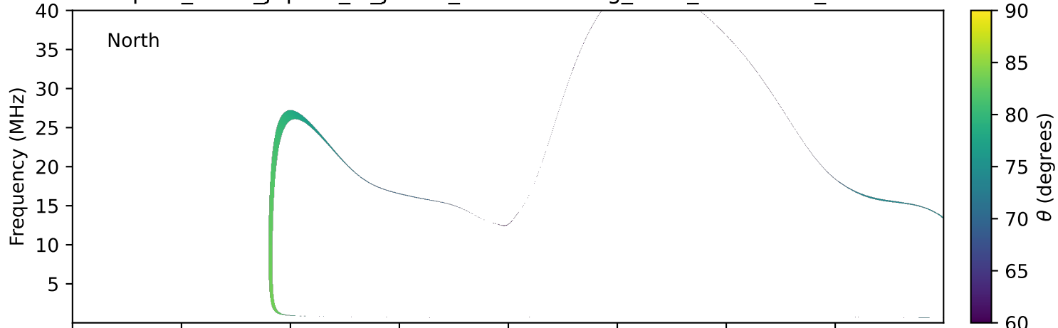
expres_earth_jupiter_io_jrm09_lossc-wid1deg_3kev_19990808_v11.cdf
