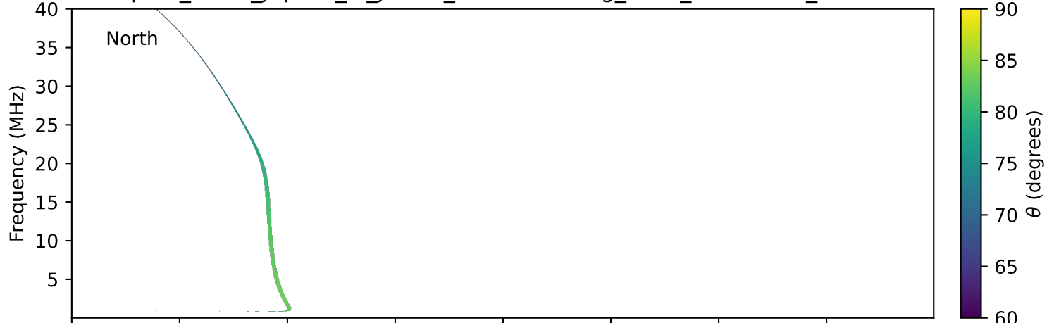
expres_earth_jupiter_io_jrm09_lossc-wid1deg_3kev_19990807_v11.cdf
