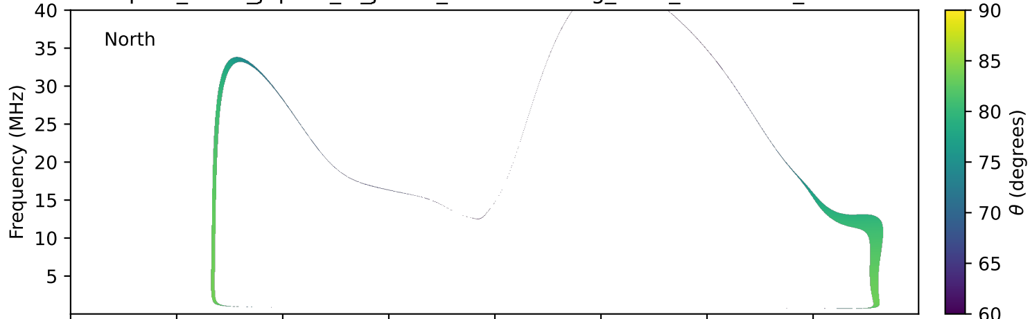
expres_earth_jupiter_io_jrm09_lossc-wid1deg_3kev_19990801_v11.cdf
