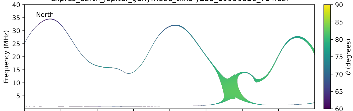
expres_earth_jupiter_ganymede_txka-y235_19990826_v14.cdf
