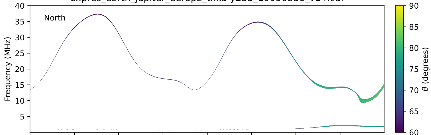
expres_earth_jupiter_europa_txka-y235_19990830_v14.cdf
