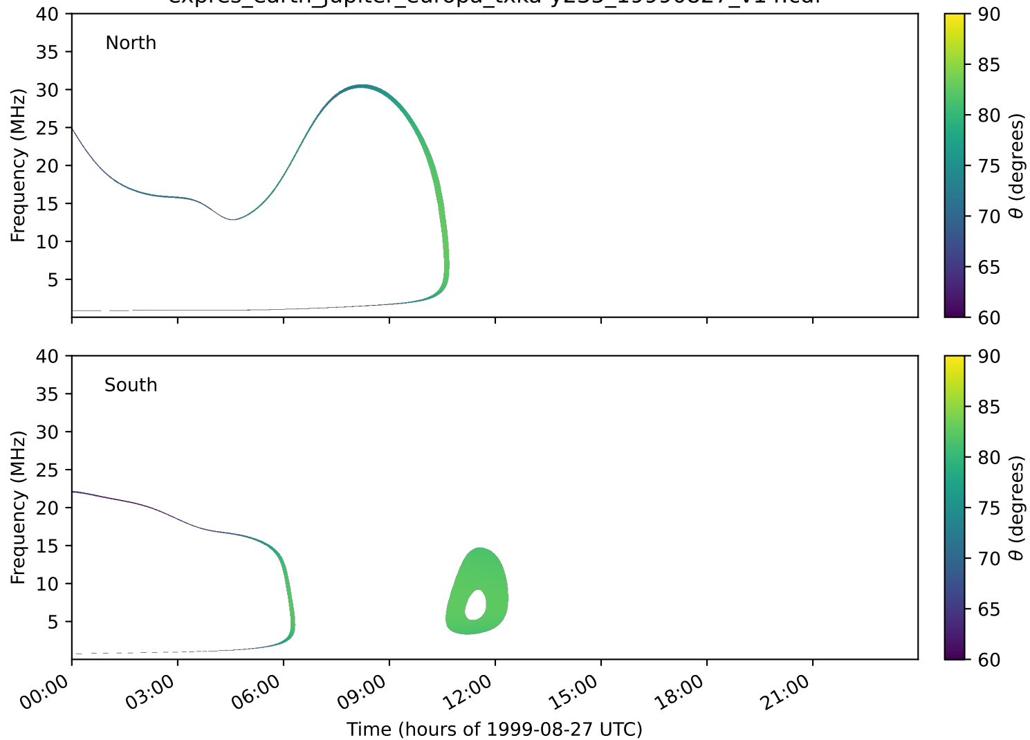
expres_earth_jupiter_europa_txka-y235_19990827_v14.cdf
