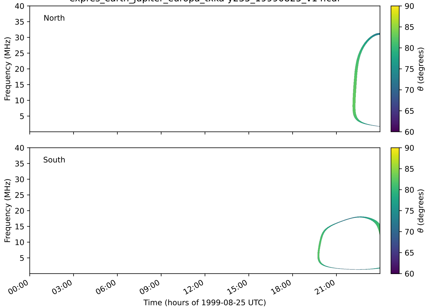
expres_earth_jupiter_europa_txka-y235_19990825_v14.cdf
