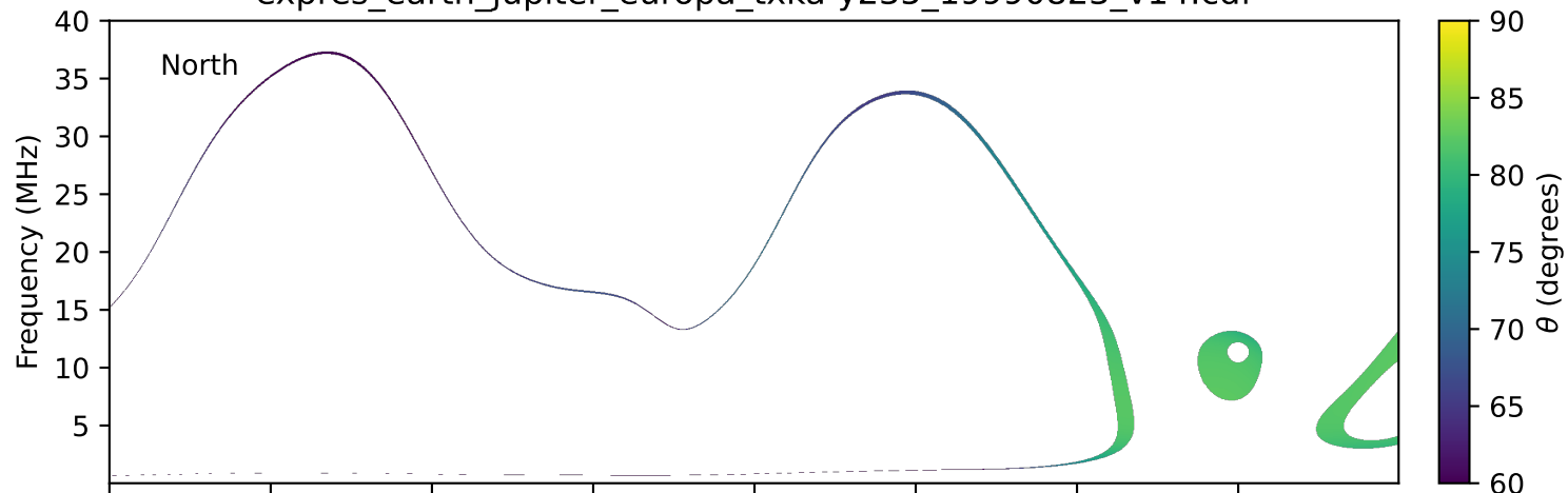
expres_earth_jupiter_europa_txka-y235_19990823_v14.cdf
